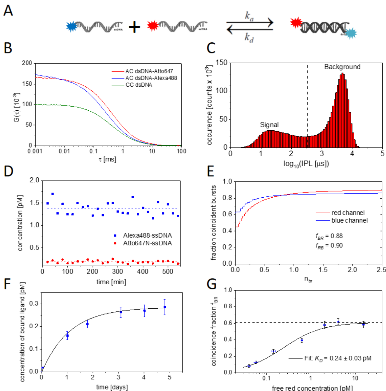
Figure 1. Experimental data illustrating the typical workflow of analysis and validation steps in a BTCCD-based measurement of a binding curve. (A) Schematic illustration of the DNA binding reaction (1:1 binding stoichiometry). The model system used here consists of 24-base-pair DNA; each complementary single strand is labeled either with Alexa488 (blue) or with Atto647N (red). (B) An FCS analysis is shown for double-labeled dsDNA molecules (see A) as measured in the nanomolar concentration regime. In addition to both autocorrelation functions (AC), each obtained for one color, the related dual-color cross-correlation (CC) is shown. (C) Example of an IPL histogram showing data from the red detection channel, taken from measurements at room temperature, with 1.5 pM
