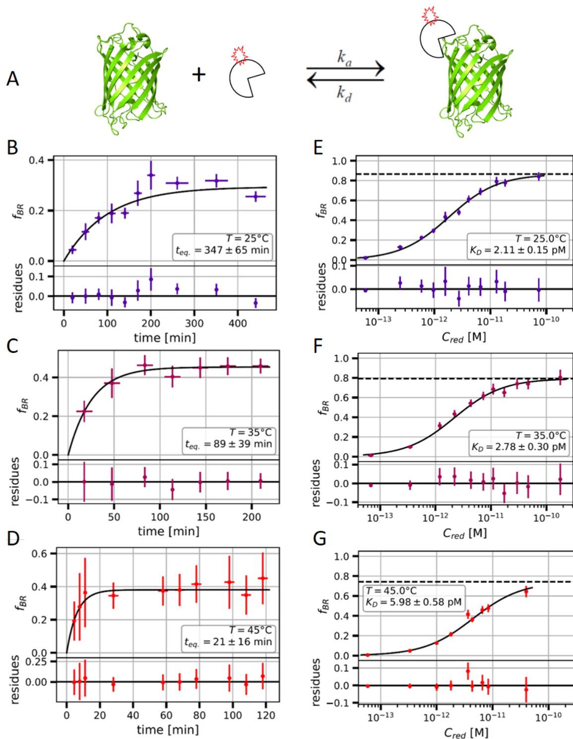
Figure 2. (A) Schematic illustration of the EGFP-nanobody binding reaction. EGFP (green) with a molecular mass of 27 kDa and the nanobody (black), MW: 14 kDa, conjugated with Atto647N (red). (B–D) Equilibrium time curves from which the fit gives equilibrium times t_{eq} = 5 \cdot t_{1/2} between ~350–20 min for reaction at temperatures between 25 and 45 °C. EGFP concentrations [B] were kept at values of 1 pM for the 25 °C sample and of 4 pM for the 45 °C sample. Hyperbolic model fits are shown for corrected [R]_{free} values calculated with f_{BR} (see E–G), while the hyperbolic model fit with corrected [R]_{free} values calculated by using f_{RB} and quadratic model fits are shown Figure S4. The dashed lines represent the f_{BR}^{max} values as obtained in each fit. All given K_D values were corrected according to Equation (12); see Section 4.4.
