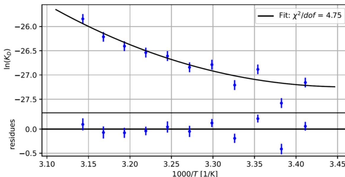
Figure 3. Van't Hoff plot with K_D values as obtained from data corrected with f_{BR} values (see Figure S4, left panels). The experimental data points (symbols) were fitted by a function (solid line) adapted from the integrated Van't Hoff equation; see Equation (18) in Section 4.5. Relevant thermodynamic parameters as obtained from the fit, as well as for the other corrected data (Figure S5), are given in Table 1.
